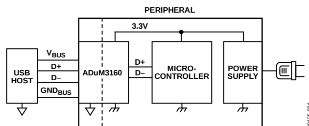
Figure 4. Typical ADuM3160 Application
